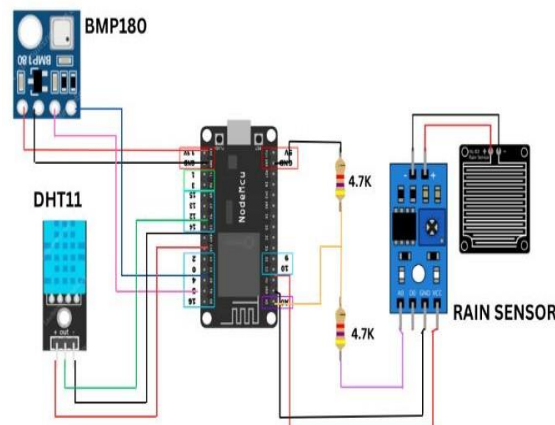
Fig 3.: Pinout of proposed model
